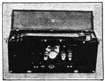
Showing location of instrument and amplifier in combination case (Patent Pending). This outfit is ideal for traveling musicians as it has room for spare tubes and accessories.
